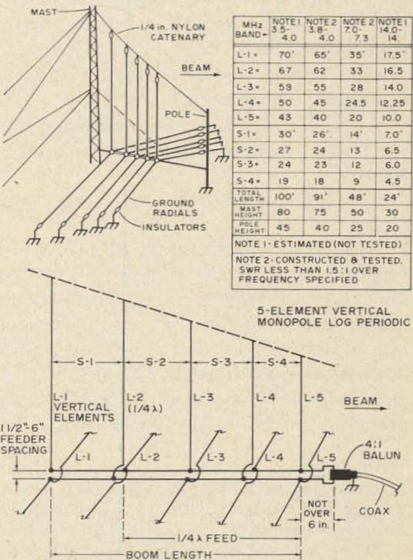
Fig. 10. 5 element vertical monopole log periodic.
